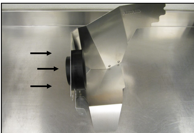
7. Install the Filter Adapter onto the Panel Assembly as shown, using the three 1/4-20 Button Head Screws and Flat Washers.
